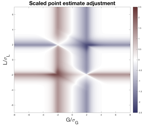
Figure 18: This figure plots the difference between the median-unbiased estimator \hat{\gamma}_{\frac{1}{2}}(X) and the conventional estimator \hat{\gamma} = G in the difference-in-differences example.
